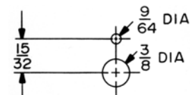
MOUNTING DIMENSIONS
